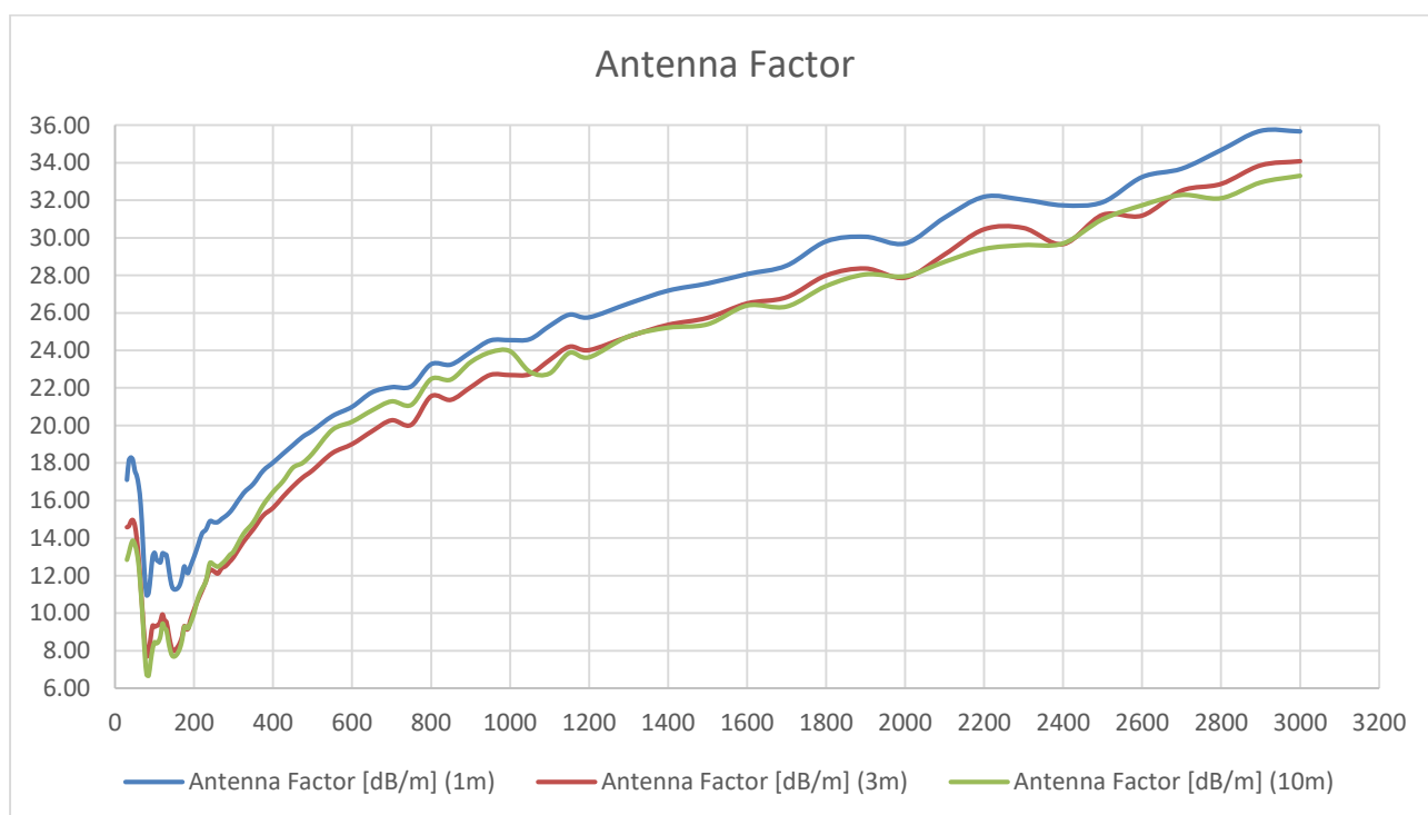
30 MHz ... 3000 MHz, Antenna Factor of TBMA8
