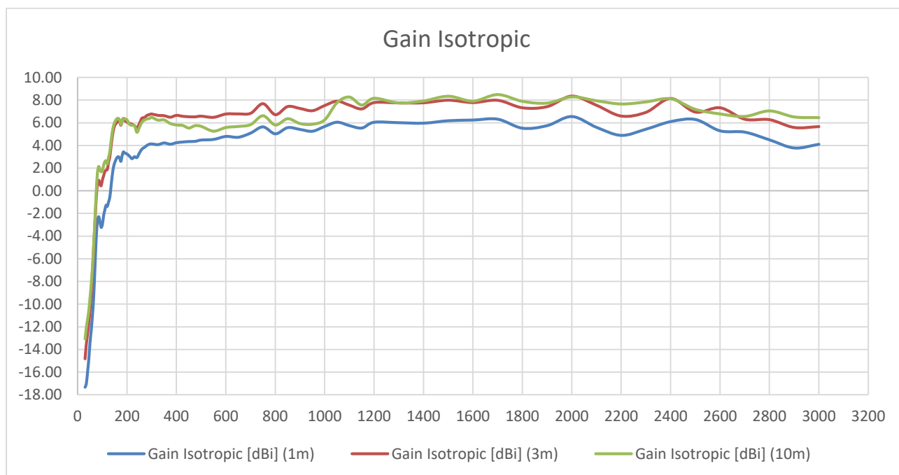
30 MHz ... 3000 MHz, Isotropic Gain of TBMA8
