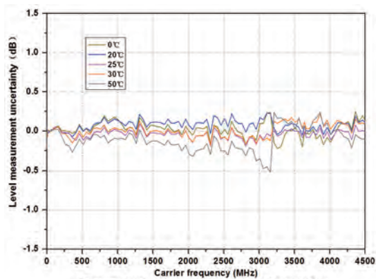
Measured level measurement uncertainty VS temperature @ -10 dBm of RSA3015N/RSA3030/RSA3030-TG/RSA3030N/RSA3045/RSA3045-TG/RSA3045N
