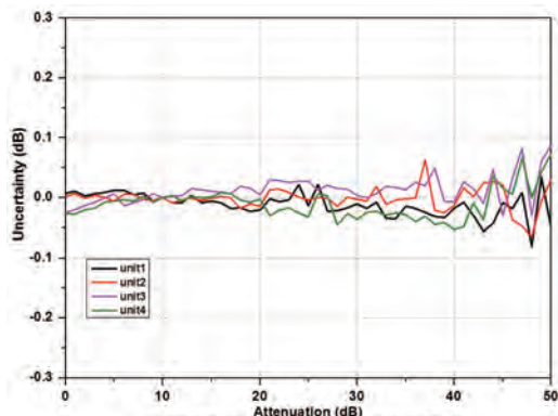
Measured attenuation switching uncertainty of RSA3015N/RSA3030/RSA3030-TG/RSA3030N/RSA3045/RSA3045-TG/RSA3045N
