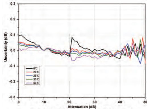
Measure attenuation switching uncertainty VS temperature of RSA3015N/RSA3030/RSA3030-TG/RSA3030N/RSA3045/RSA3045-TG/RSA3045N
