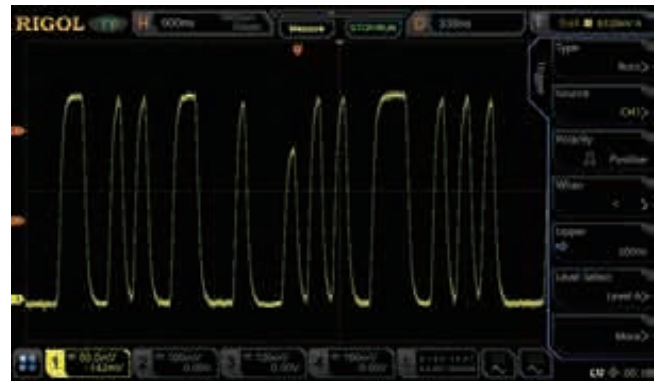
The Runt trigger helps you capture the runt pulse signal in the pulse train
