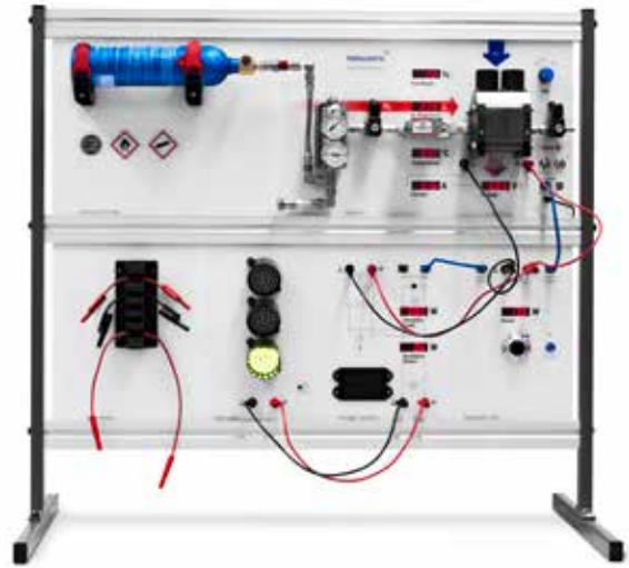
50W Fuel Cell Training System
